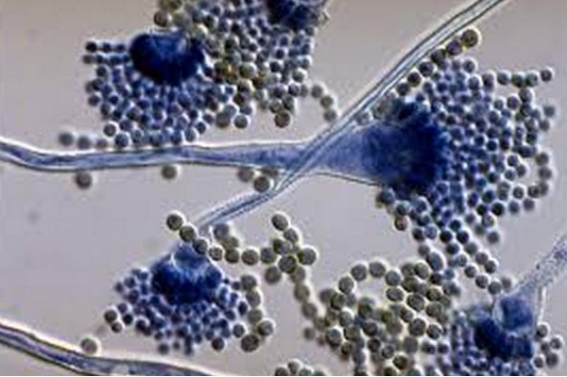
Aspergillus sp
