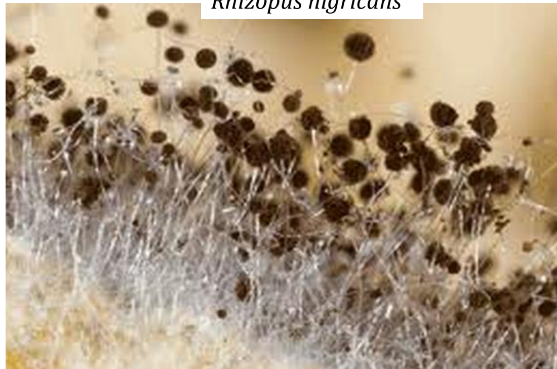
Rhizopus nigricans
