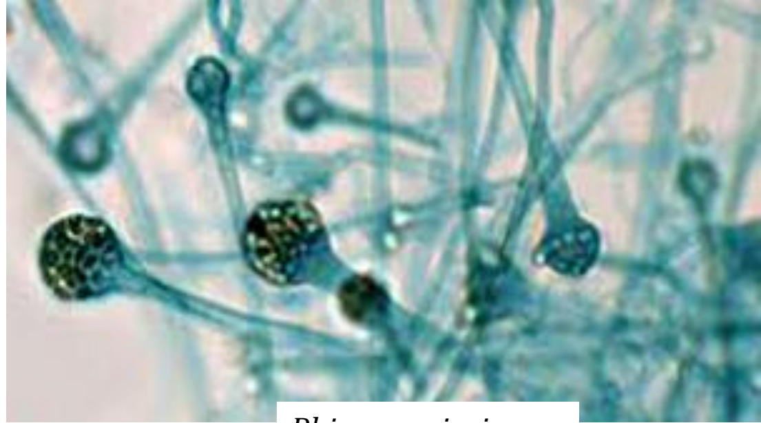
Rhizopus nigricans
